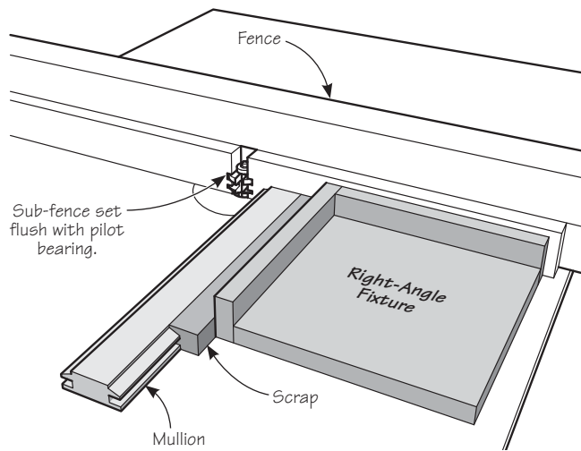
Figure 10: Using a right-angle fixture.
