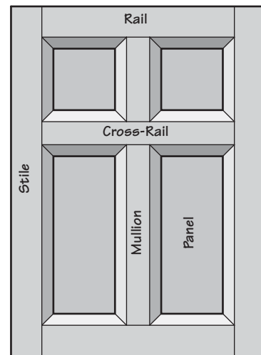
Figure 3: Door parts.
